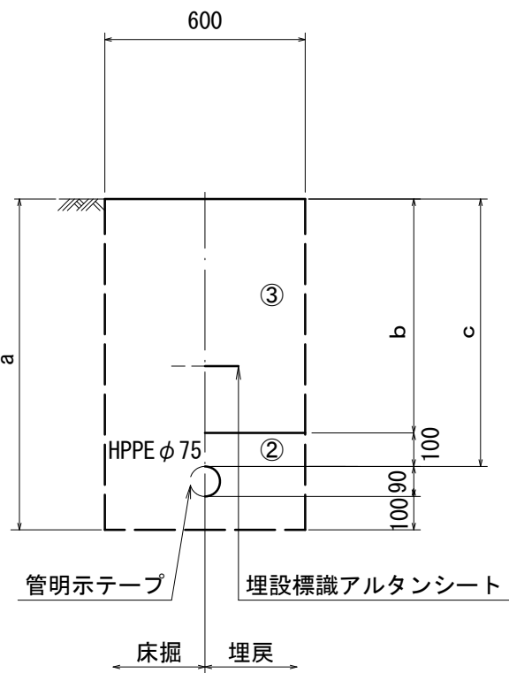
HPPEφ75
